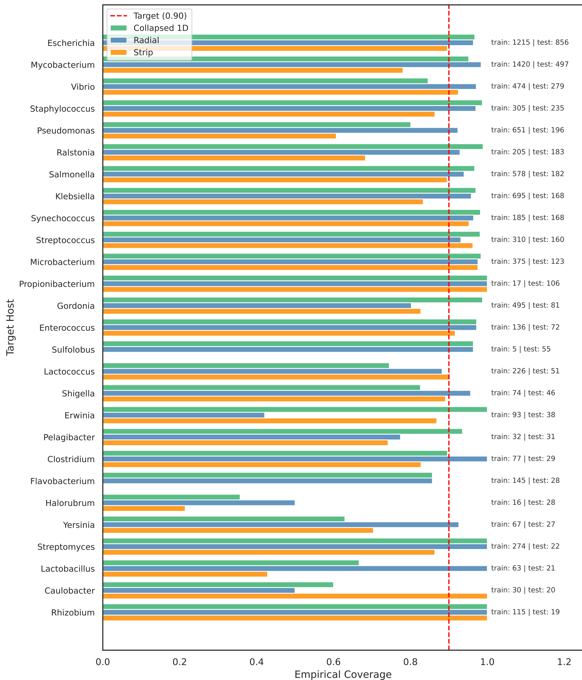
Class Conditional Coverage Breakdown Per Host (AllMethods)
